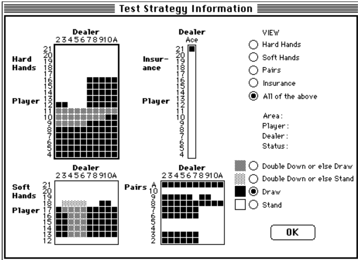
Fig. 6 Test Strategy Information Dialog
