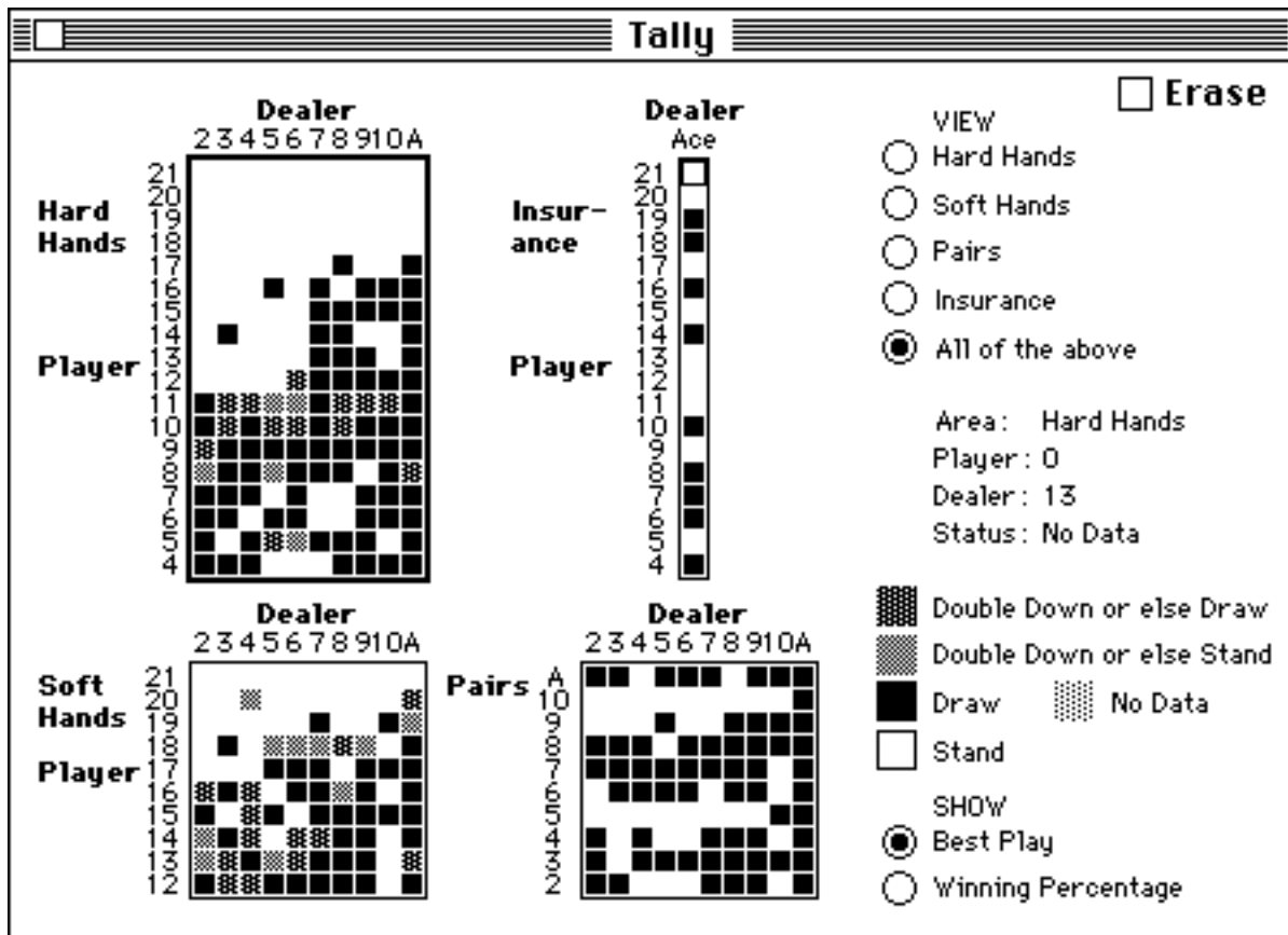
Fig. 18 Tally Window -- View All
